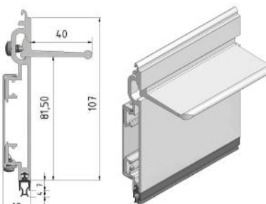
End section F1A5/FAD3/FAW5
