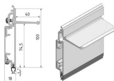
End section F1A6/FAD3/FAW5
